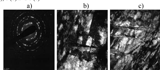
Fig. 2. Diffraction pattern and structure of steel AISI 316 after ECAP. (Log. deformation: 8)
