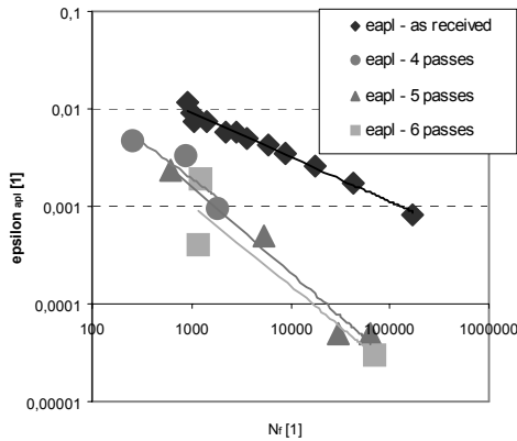
Fig. 4. Curves of low-cycle fatigue \epsilon_{apl} - N_f
