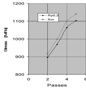
Fig. 3. Influence of number of passes on strength properties of steel AISI 316
