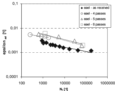
Fig. 5. Curves of low-cycle fatigue \epsilon_{ael} - N_f
