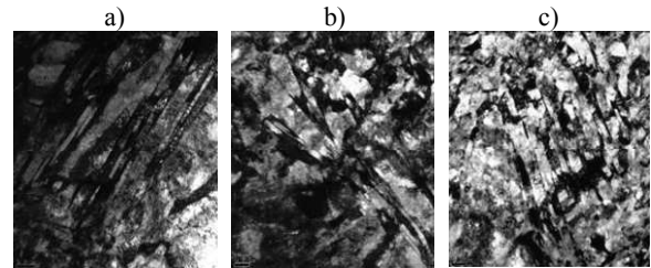
Fig. 1. Structure of steel AISI 316 after ECAP. Logarithmic deformation: 4 (a), 6 (b) and 8 (c)
