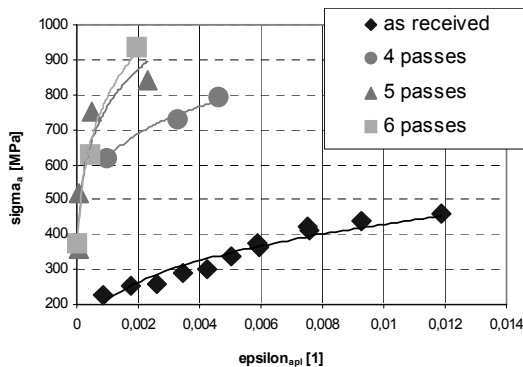
Fig. 6. Curves of dependence between the amplitude of stress \sigma_a - \epsilon_{apl}
