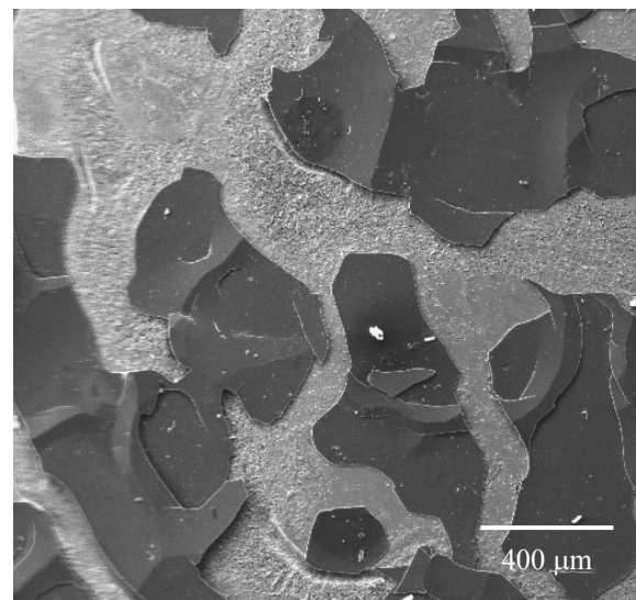
Fig. 35. Effect of the electrochemical corrosion on the Ti/TiAlN×1 coating
