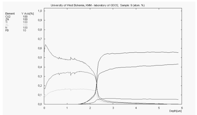
Fig. 26. Changes of constituent concentration of the Ti/TiAlN \times 150 and the substrate materials
