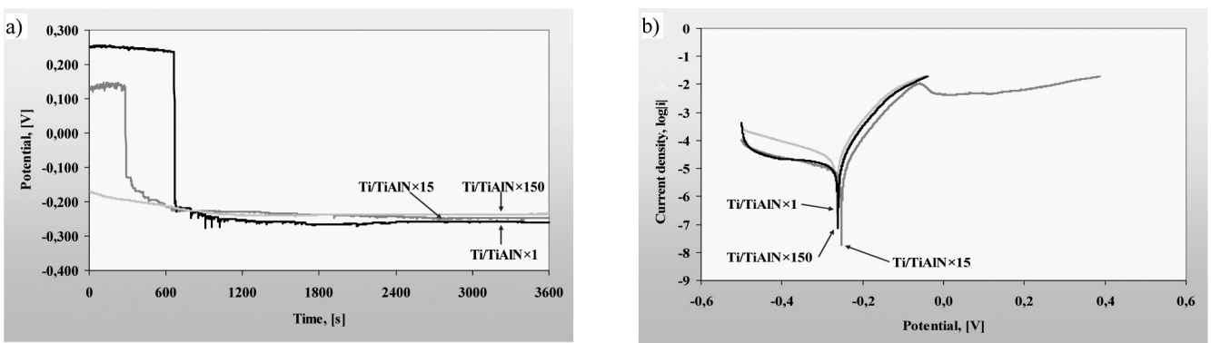
Fig. 31. a) Open circuit potential curves, b) potentiodynamic polarization curves of the Ti/TiAlN coatings in 1 M HCl solution
