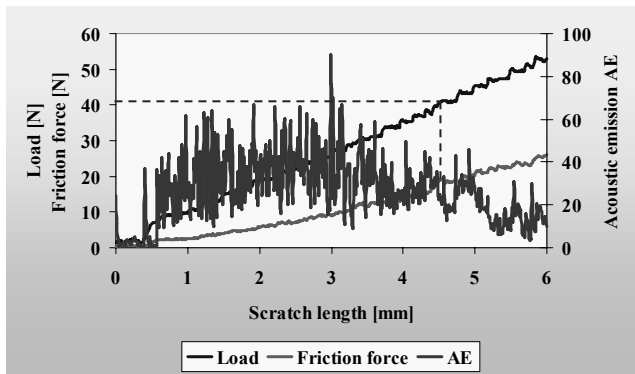
Fig. 37. Diagram of the dependence of the acoustic emission (AE) and friction force F_t on the load for the Ti/ZrN \times 15 coating
