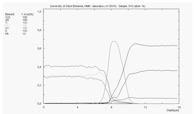
Fig. 27. Changes of constituent concentration of the Mo/TiAlN \times 1 and the substrate materials
