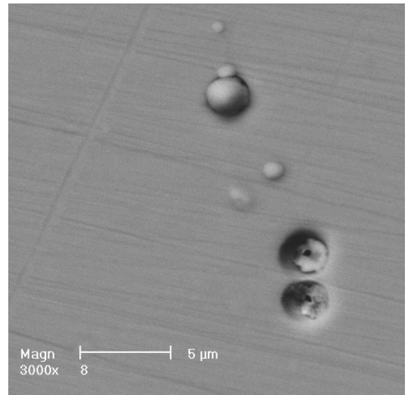
Fig. 12. Topography of the Ti/ZrN \times 15 coating surface deposited onto the CuZn40Pb2 brass substrate
