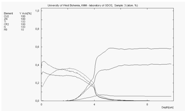
Fig. 20. Changes of constituent concentration of the Ti/CrN×150 and the substrate materials
