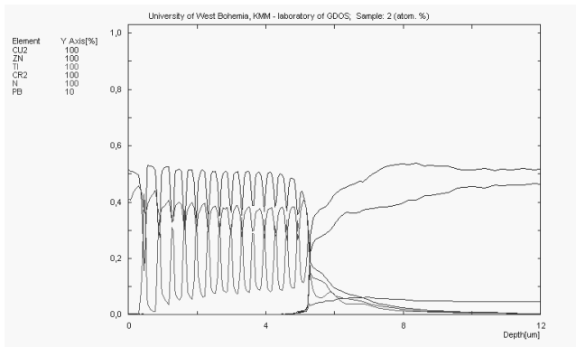
Fig. 19. Changes of constituent concentration of the Ti/CrN×15 and the substrate materials
