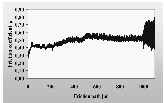
Fig. 46. Plot of the friction coefficient depending on friction path for the pin-on-disc of the Ti/CrN x 15 coating
