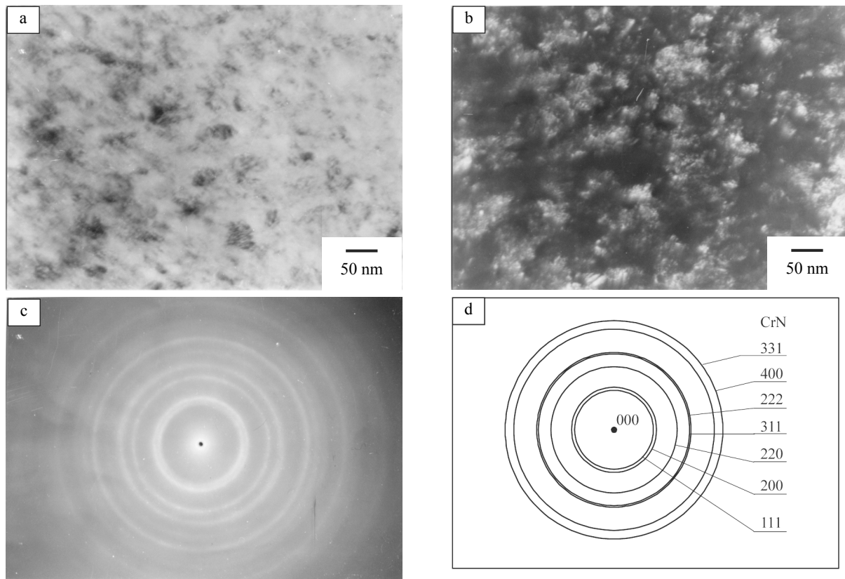
Fig. 14. Structure of the thin foil from the Ti/CrN \times 1 coating deposited onto CuZn40Pb2 brass substrate, a) light field, b) dark field from the {111} reflex, c) diffraction pattern from the area as in a, d) solution of the diffraction pattern
