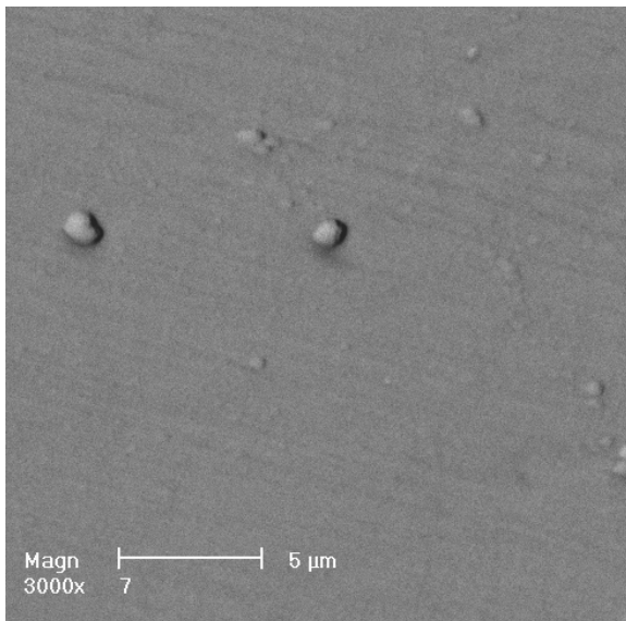
Fig. 11. Topography of the Ti/ZrN \times 1 coating surface deposited onto the CuZn40Pb2 brass substrate
