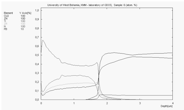
Fig. 23. Changes of constituent concentration of the Ti/ZrN \times 150 and the substrate materials
