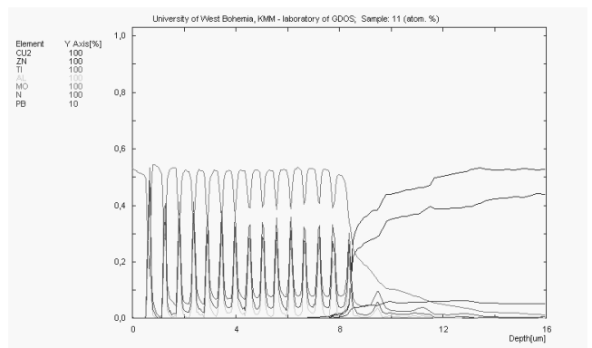
Fig. 28. Changes of constituent concentration of the Mo/TiAlN \times 15 and the substrate materials
