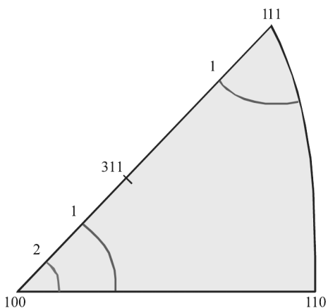
Fig. 16. Inverse pole figures representing the distribution of the normal to the Ti/CrN×15 coating surface in the 001-011-111 base triangle
