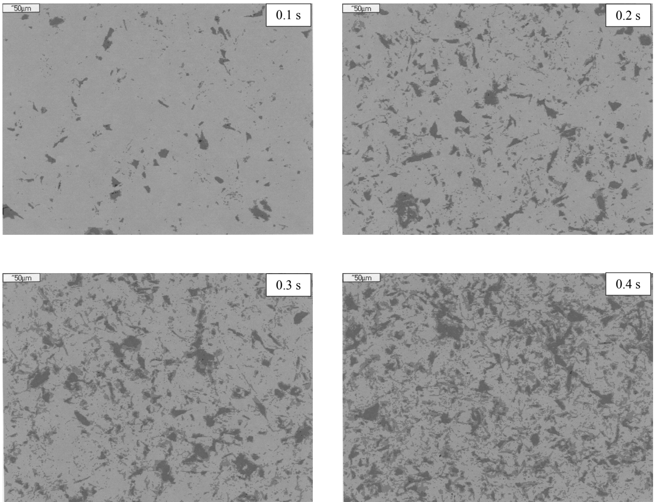
Fig. 40. Surface of the Ti/ZrN \times 1 coating in various of the erosion test stages, depending on the SEM test duration
