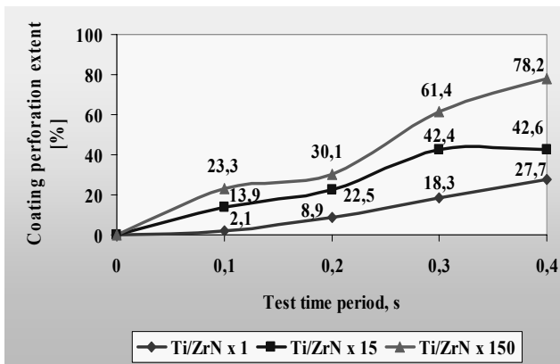
Fig. 43. Extent of perforation of the Ti/ZrN coatings deposited onto the CuZn40Pb2 substrate depending on the erosion test time period
