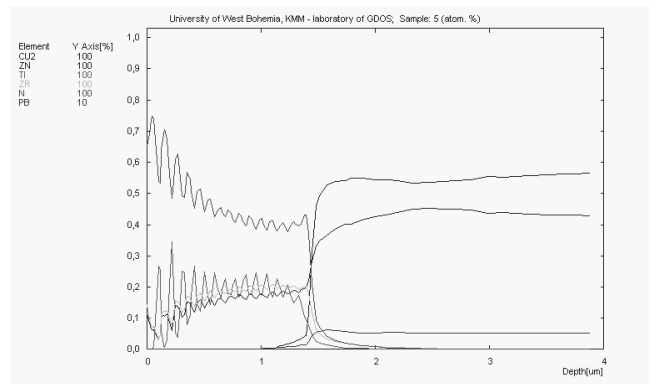
Fig. 22. Changes of constituent concentration of the Ti/ZrN×15 and the substrate materials
