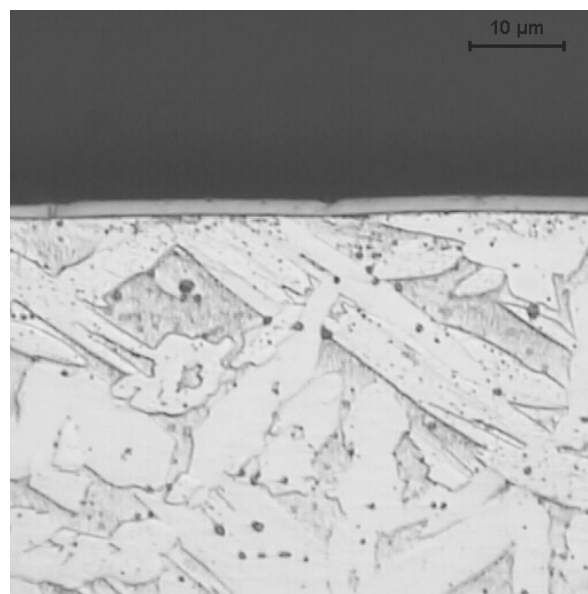
Fig. 5. Mo/TiAlN \times 1 coating deposited onto the CuZn40Pb2 substrate
