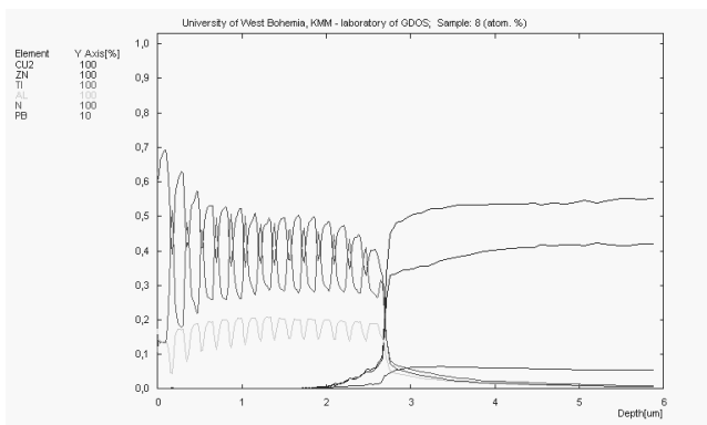
Fig. 25. Changes of constituent concentration of the Ti/TiAlN \times 15 and the substrate materials
