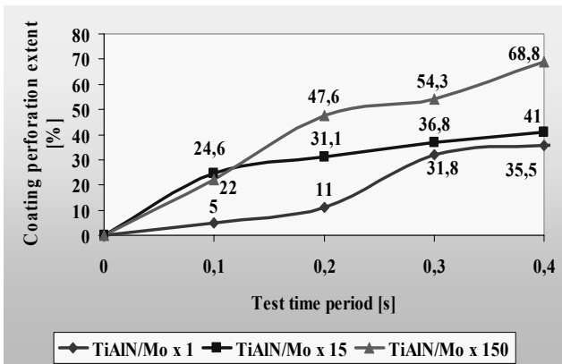
Fig. 44. Extent of perforation of the Mo/TiAlN coatings deposited onto the CuZn40Pb2 substrate depending on the erosion test time period
