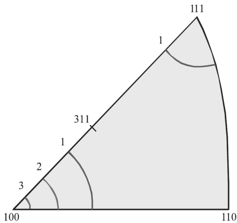
Fig. 15. Inverse pole figures representing the distribution of the normal to the Ti/CrN×1 coating surface in the 001-011-111 base triangle
