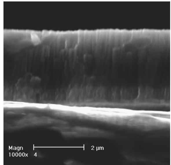
Fig. 8. Fracture of the Ti/TiAlN×1 coating deposited onto the CuZn40Pb2 brass substrate
