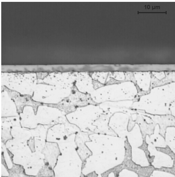
Fig. 6. Mo/TiAlN×15 coating deposited onto the CuZn40Pb2 substrate
