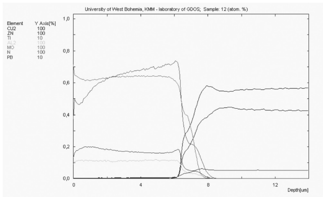
Fig. 29. Changes of constituent concentration of the Mo/TiAlN \times 150 and the substrate materials
