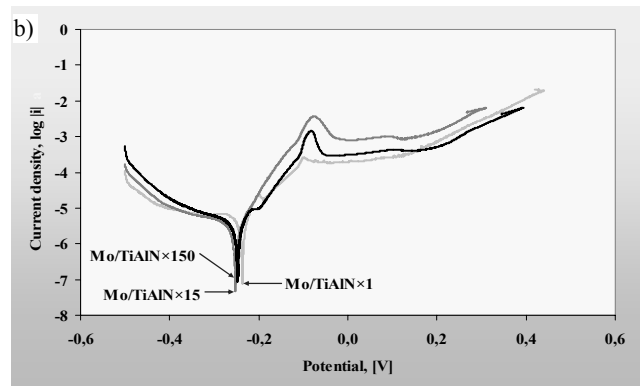
Fig. 33. a) Open circuit potential curves, b) potentiodynamic polarization curves of the Mo/TiAlN coatings in 1 M HCl solution
