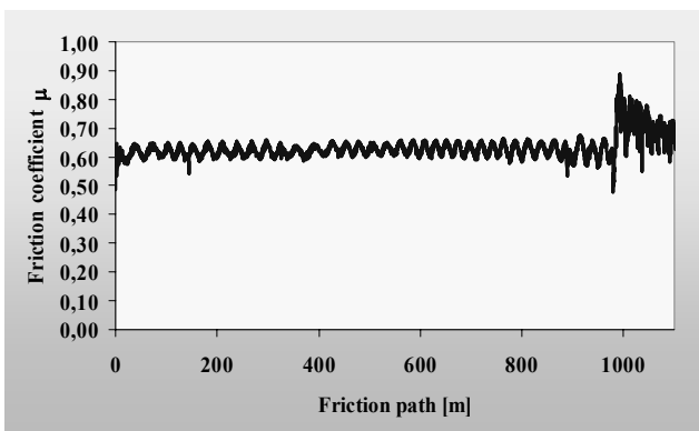
Fig. 45. Plot of the friction coefficient depending on friction path for the pin-on-disc of the Ti/CrN x 1 coating
