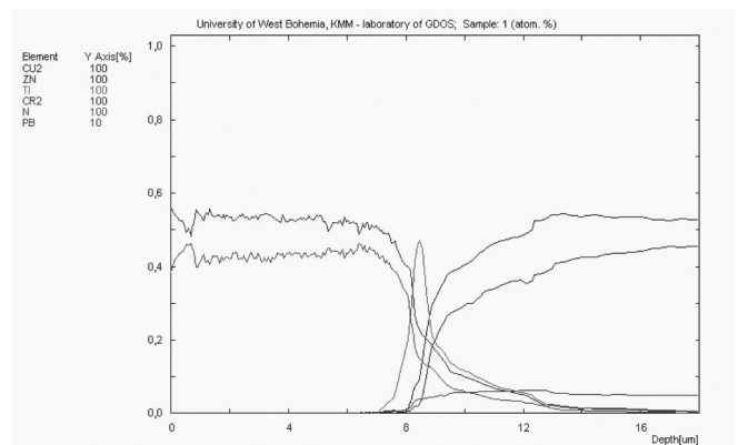
Fig. 18. Changes of constituent concentration of the Ti/CrN×1 and the substrate materials
