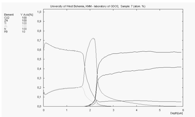
Fig. 24. Changes of constituent concentration of the Ti/TiAlN \times 1 and the substrate materials
