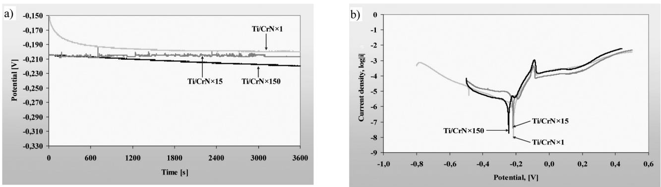
Fig. 30. a) Open circuit potential curves, b) potentiodynamic polarization curves of the Ti/CrN coatings in 1 M HCl solution
