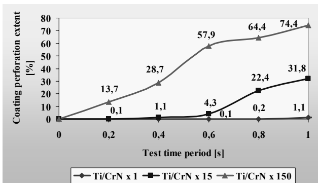
Fig. 41. Extent of perforation of the Ti/CrN coatings deposited onto the CuZn40Pb2 substrate depending on the erosion test time period
