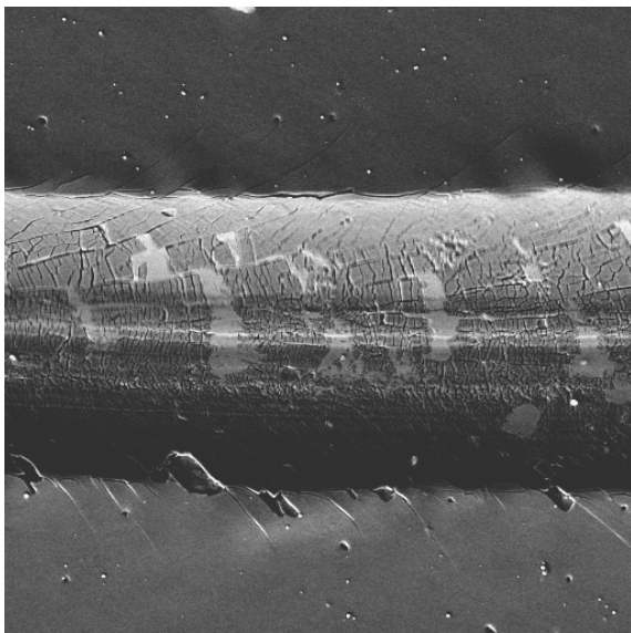
Fig. 39. Characteristic failure of the Ti/CrN \times 1 coating developed during the scratch test, SEM
