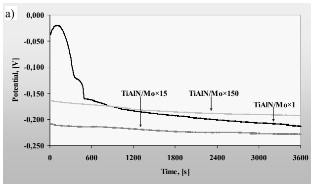
Fig. 33. a) Open circuit potential curves, b) potentiodynamic polarization curves of the Mo/TiAlN coatings in 1 M HCl solution
