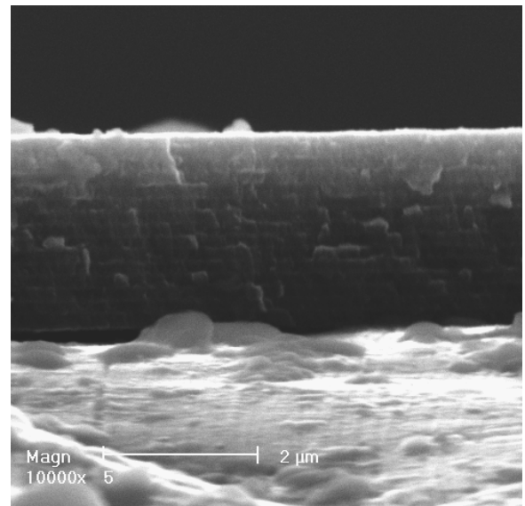
Fig. 9. Fracture of the Ti/TiAlN×15 coating deposited onto the CuZn40Pb2 brass substrate
