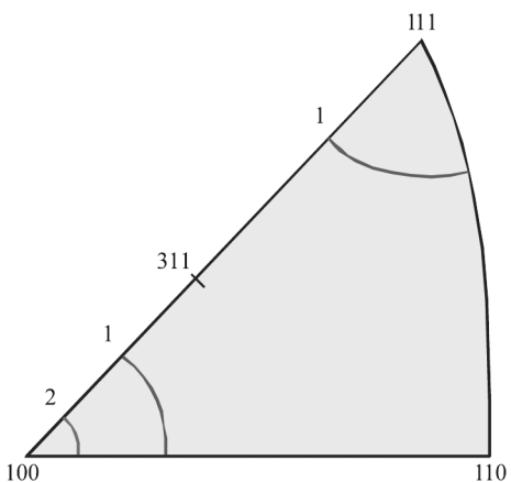
Fig. 17. Inverse pole figures representing the distribution of the normal to the Ti/CrN×150 coating surface in the 001-011-111 base triangle
