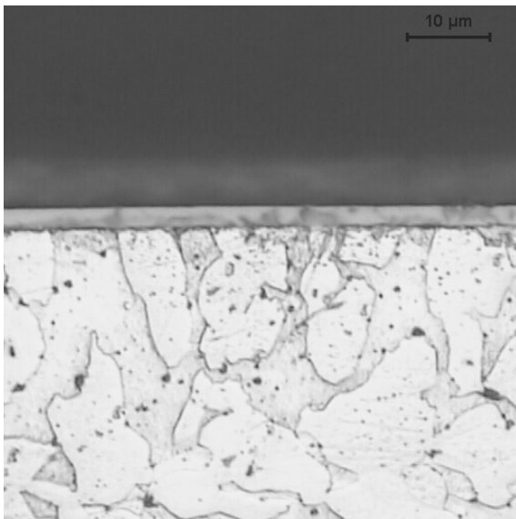
Fig. 7. Mo/TiAlN×150 coating deposited onto the CuZn40Pb2 substrate
