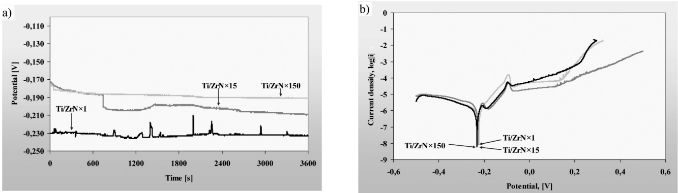
Fig. 32. a) Open circuit potential curves, b) potentiodynamic polarization curves of the Ti/ZrN coatings in 1 M HCl solution
