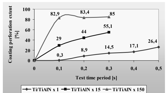
Fig. 42. Extent of perforation of the Ti/TiAlN coatings deposited onto the CuZn40Pb2 substrate depending on the erosion test time period
