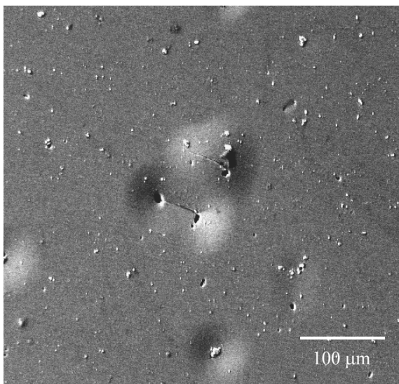
Fig. 34. Effect of the electrochemical corrosion on the Ti/CrN×15 coating
