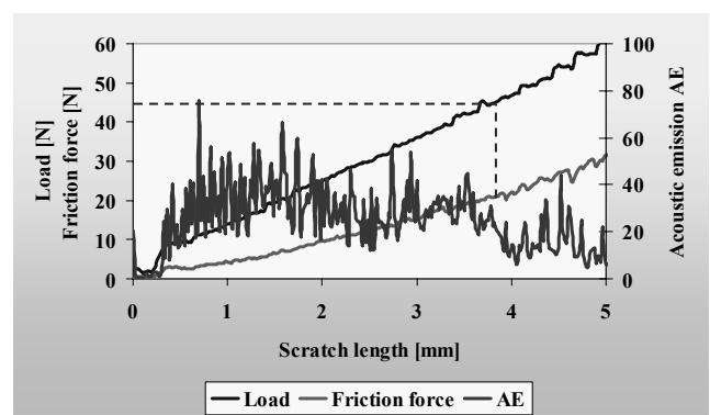
Fig. 36. Diagram of the dependence of the acoustic emission (AE) and friction force F_t on the load for the Ti/ZrN×1 coating
