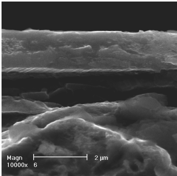
Fig. 10. Fracture of the Ti/TiAlN \times 150 coating deposited onto the CuZn40Pb2 brass substrate
