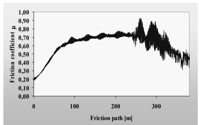
Fig. 47. Plot of the friction coefficient depending on friction path for the pin-on-disc of the Ti/CrN x 150 coating
