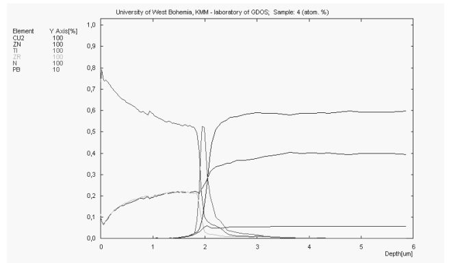
Fig. 21. Changes of constituent concentration of the Ti/ZrN×1 and the substrate materials
