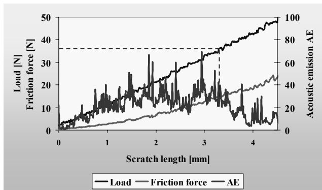
Fig. 38. Diagram of the dependence of the acoustic emission (AE) and friction force F_t on the load for the Ti/ZrN \times 15 coating
