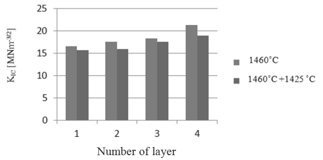
Fig. 52. Brittle cracking co-efficient diagram according to temperature and fraction volume of Co for four layers of GM-3Co/97WC sintered in a vacuum furnace
