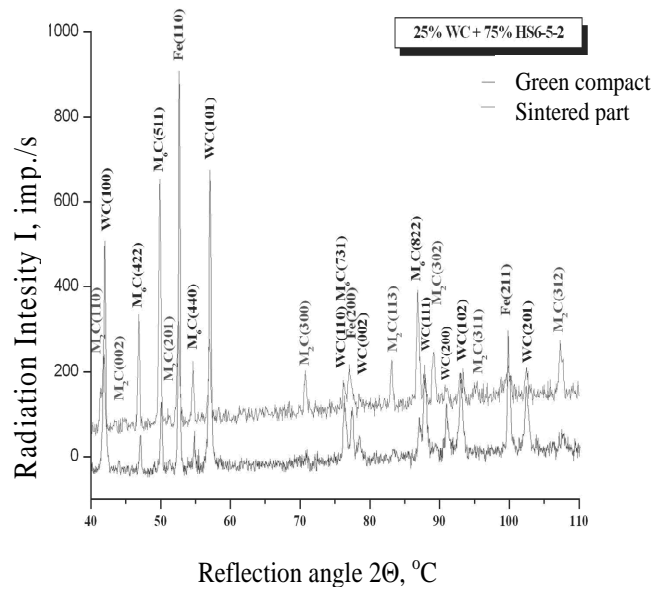
Fig. 28. Results of the X-ray phase analysis for the sintered test piece with the 75HSS/25WC surface layer; diffraction patterns were shifted along the vertical axis to show the results more clearly
