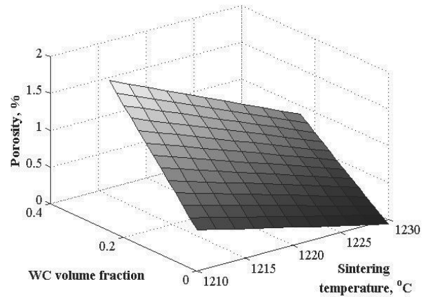
Fig. 24. RFP describing relationship between porosity and the volume fraction of the reinforcing phase and sintering temperature, for GM-HSS/WC sintered in a vacuum furnace for 30 min
