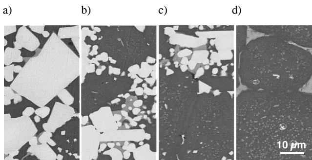
Fig. 32. Layers structure of GM-75HSS/25WC sintered in a vacuum furnace at the temperature of 1230°C, for 60 min; a) surface layer, b),c) intermediate layers, d) substrate layer
