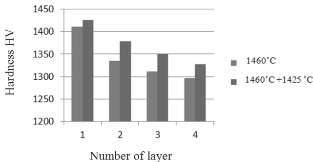
Fig. 51. Diagram of HV hardness, fraction volume and sintering temperature for four layers of GM-3Co/97WC
