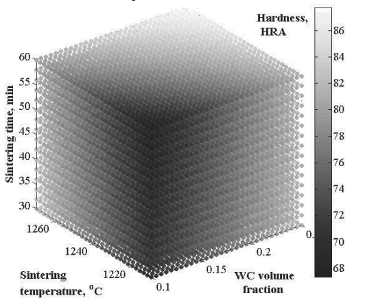
Fig. 14. RFP describing relationship between hardness and WC volume fraction, temperature, and sintering time, for GM-HSS/WC sintered in a vacuum furnace
