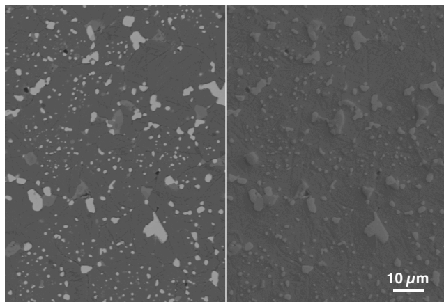
Fig. 42. Structure of the quenched and twice tempered GM-100HSS substrate layer of GM-75HSS/25WC
