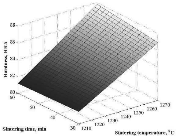
Fig. 16. RFP describing relationship between hardness and the temperature, and sintering time, for GM-75HSS/25WC sintered in a vacuum furnace
