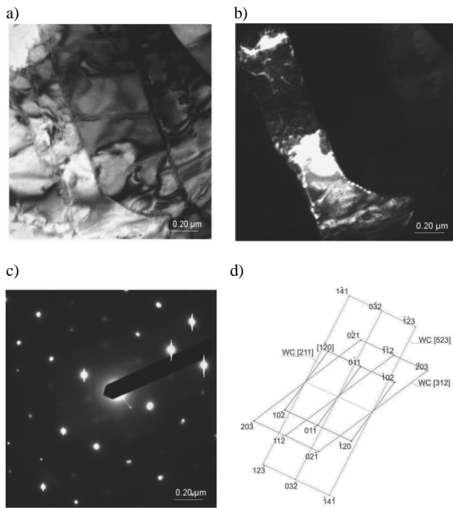
Fig. 50. The structure of thin foils made of WC-Co sintered carbide after sintering at the temperature of 1460°C; a) image in the light field; b) image in the dark field of Co and WC; c) diffraction pattern from the area as in figure a; d) diffraction pattern solution from figure c [58]
