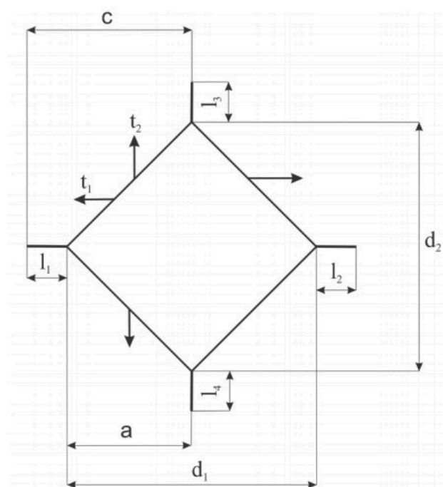
Fig. 7. Diagram of cracks system obtained with the Palmqvist method
