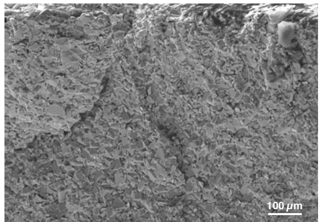
Fig. 53. Fracture structure of the GM-3Co/97WC surface layer sintered in a vacuum furnace at the temperature of 1460°C
