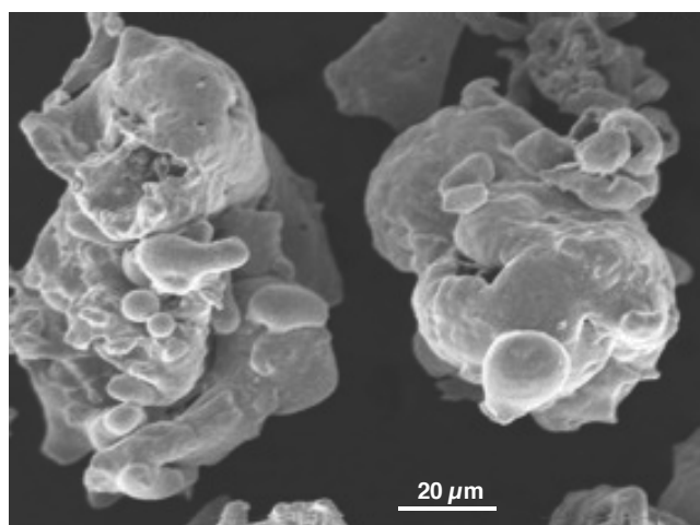
Fig. 2. A scanning electron micrograph of HS6-5-2 water atomized powders
