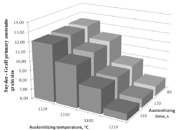
Fig. 45. Relationship between the primary austenite grain size in the GM-100HSS substrate layer of hardened GM-75HSS/25WC and austenitising conditions
