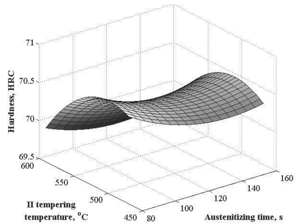
Fig. 38. RFP describing relationship between hardness and the second tempering temperature, and austenitising time, for the GM-75HSS/25WC surface layer austenitised at the temperature of 1150°C
