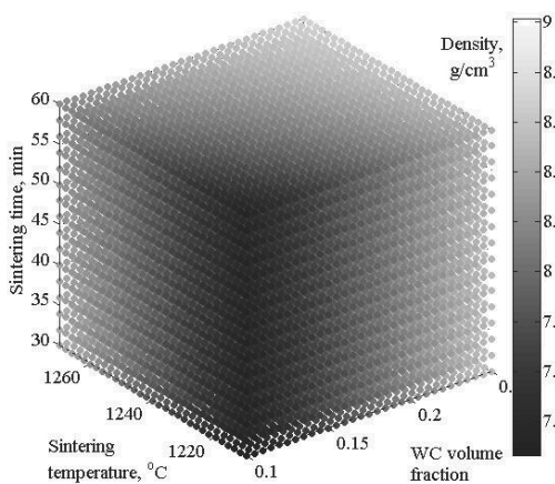
Fig. 8. RFP describing relationship between density and the WC volume fraction, temperature, and sintering time, for GM-HSS/WC sintered in a vacuum furnace
