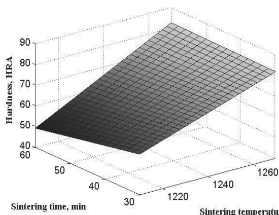
Fig. 18. RFP describing relationship between hardness and the temperature, and sintering time, for GM-90HSS/10WC, sintered in the furnace with the atmosphere of the flowing N_2+5\% H_2
