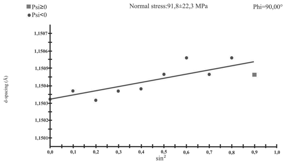
Fig. 57. Changes in the interplanar distance value of d reflex (201) according to \sin^2\psi sintering temperature of 1460°C; results for the GM-9Co/91WC substrate layer
