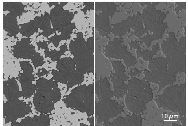
Fig. 40. Structure of the quenched and twice tempered GM-85HSS/15WC intermediate layer
