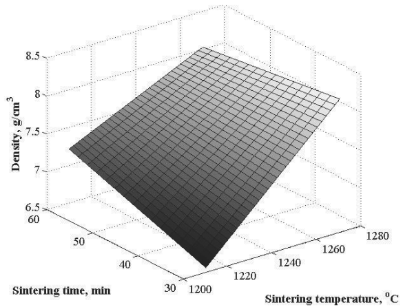
Fig. 13. RFP describing relationship between density and the temperature, and sintering time, for GM-75HSS/25WC, sintered in furnace with the atmosphere of the N_2+5\% H_2
