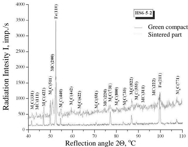
Fig. 27. Results of the X-ray phase analysis for the sintered test piece with the HS6-5-2 layer; diffraction patterns were shifted along the vertical axis to show the results more clearly
