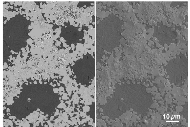
Fig. 39. Structure of the quenched and twice tempered GM-75HSS/25WC surface layer
