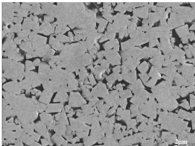
Fig. 48. Structure of the GM-3Co/97WC surface layer sintered in a vacuum furnace at the temperature of 1460°C
