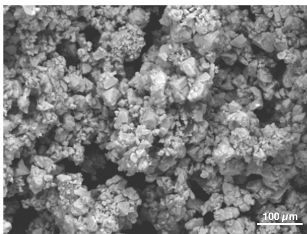
Fig. 5. Mixture of WC (93%) and Co (7%) powder after 8 hours of crushing in a ball mill
