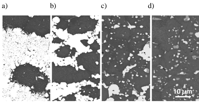
Fig. 31. Layers structure of GM-75HSS/25WC sintered in a vacuum furnace at the temperature of 1210°C, for 30 min; a) surface layer, b),c) intermediate layers, d) substrate layer
