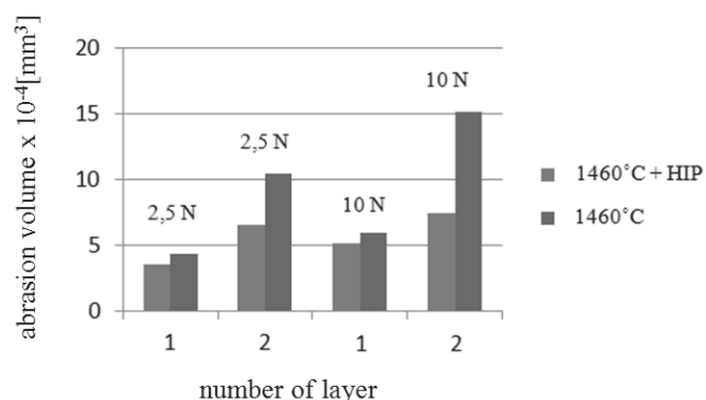
Fig. 54. Tribological wear of investigated GM-3Co/97WC
