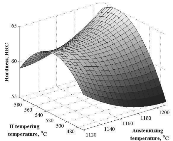
Fig. 34. RFP describing relationship between hardness and the second tempering temperature, and the austenitising temperature, for the GM-100HSS substrate layer of GM-75HSS/25WC austenitised for 120 s
