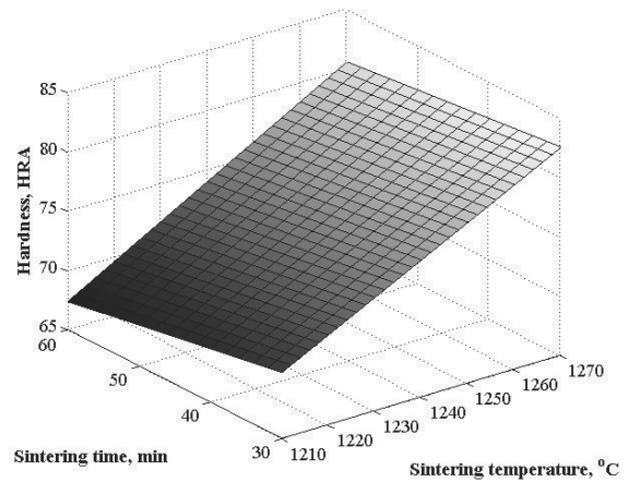
Fig. 15. RFP describing relationship between hardness and the temperature, and sintering time, for GM-90HSS/10WC sintered in a vacuum furnace
