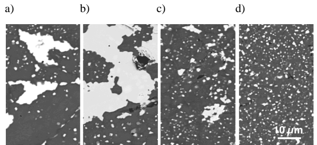
Fig. 29. Layers structure of GM-90HSS/10WC sintered in a vacuum furnace at the temperature of 1210°C, for 30 min; a) surface layer, b), c) intermediate layers, d) substrate layer
