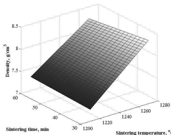
Fig. 9. RFP describing relationship between density and the temperature, and sintering time, for GM-90HSS/10WC, sintered in the vacuum furnace
