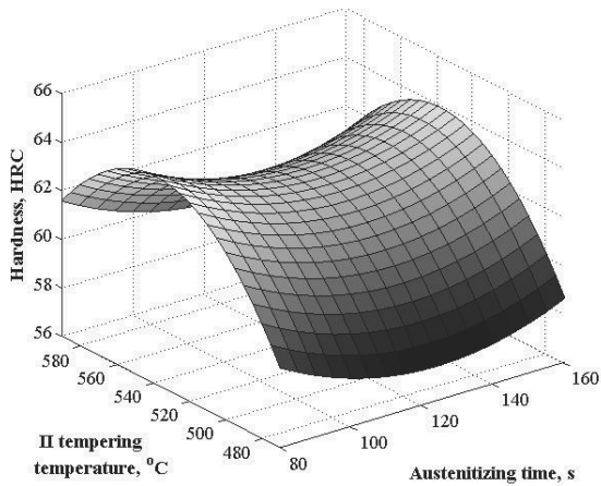
Fig. 35. RFP describing relationship between hardness and the second tempering temperature, and the austenitising time, for the GM-100HSS substrate layer of GM-75HSS/25WC austenitised at the temperature of 1150°C
