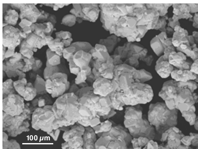
Fig. 3. A scanning electron micrograph of WC powders
