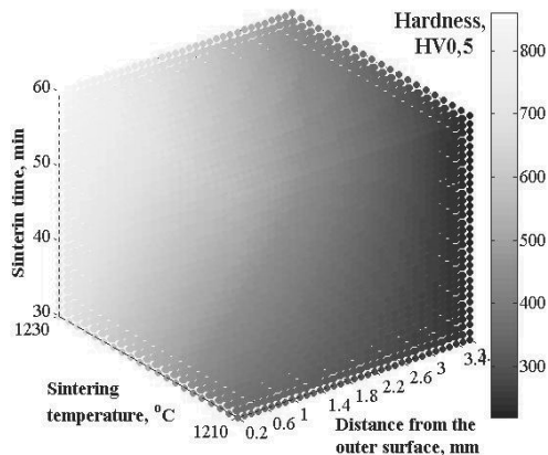
Fig. 23. RFP describing relationship between hardness HV and the distance from the outer surface, temperature, and sintering time, for GM-75HSS/25WC, sintered in the furnace with the atmosphere of the flowing N_2+5\% H_2
