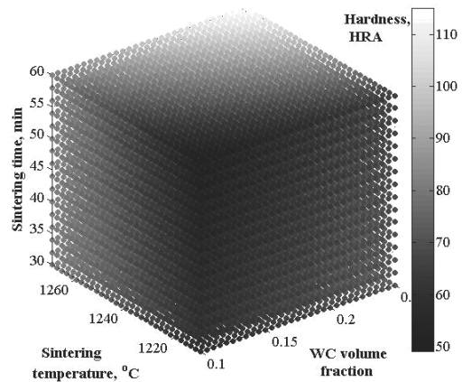
Fig. 17. RFP describing relationship between hardness and WC volume fraction, temperature, and sintering time, for GM-HSS/WC, sintered in the furnace with the atmosphere of the flowing N_2+5\% H_2
