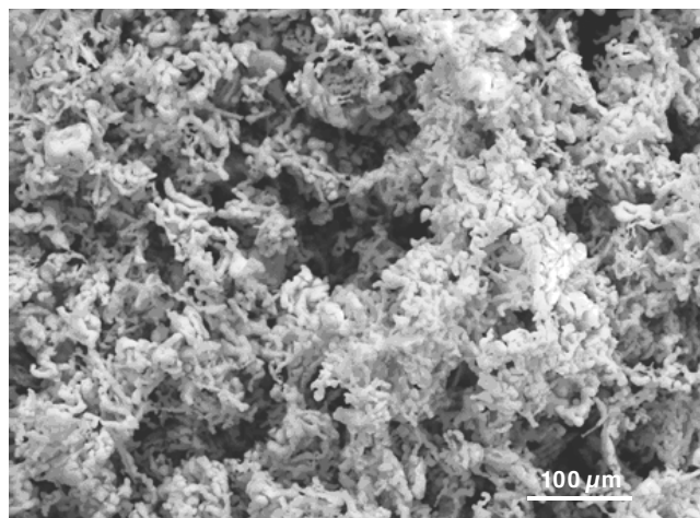
Fig. 4. A scanning electron micrograph of Co powders
