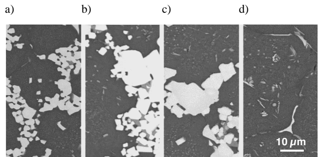
Fig. 30. Layers structure of GM-90HSS/10WC sintered in a vacuum furnace at the temperature of 1270°C, for 60 min; a) surface layer, b), c) intermediate layers, d) substrate layer
