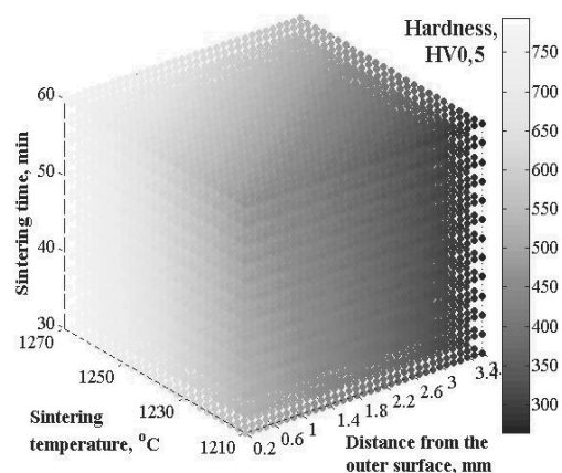
Fig. 20. RFP describing relationship between hardness HV and the distance from the outer surface, temperature, and sintering time, for GM-90HSS/10WC sintered in a vacuum furnace
