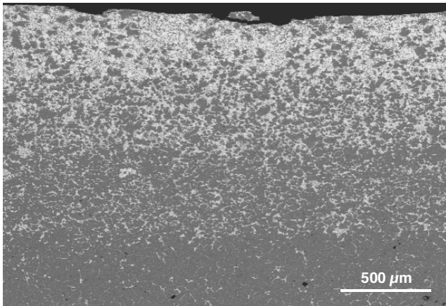
Fig. 26. Microstructures of GM-90HSS/10WC sintered in the vacuum furnace at the temperature of 1230°C, for 30 min
