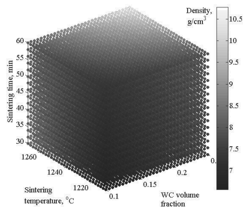
Fig. 11. RFP describing relationship between density and the WC volume fraction, temperature, and sintering time, for GM-HSS/WC, sintered in furnace with the atmosphere of the N_2+5\% H_2
