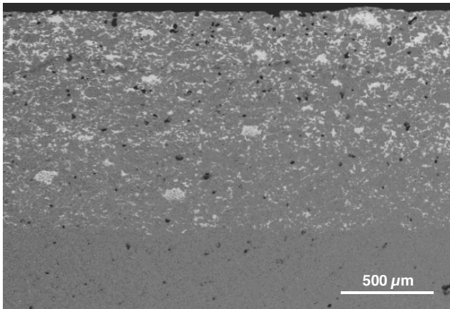
Fig. 25. Microstructures of GM-90HSS/WC sintered in the vacuum furnace at the temperature of 1230°C, for 30 min
