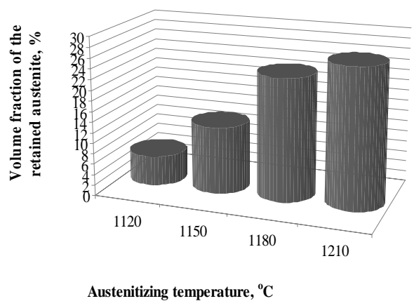
Fig. 46. Relationship between the volume portion of the retained austenite and austenitising temperature in the GM-100HSS substrate layer of hardened GM-75HSS/25WC austenitised for 120 s
