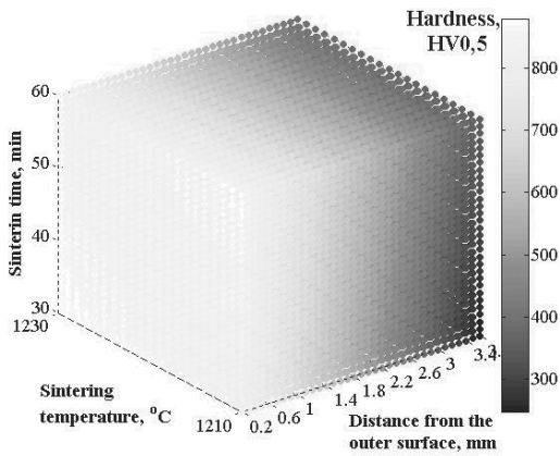
Fig. 21. RFP describing relationship between hardness HV and the distance from the outer surface, temperature, and sintering time, for GM-75HSS/25WC sintered in a vacuum furnace
