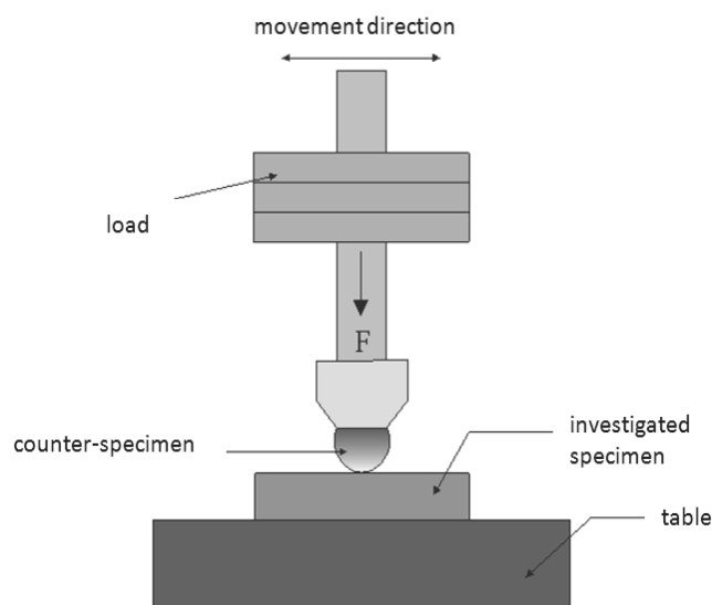
Fig. 6. Diagram of the abrasive wear resistance testing device
