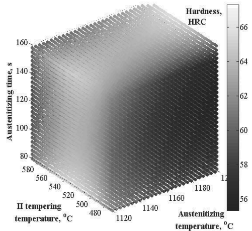
Fig. 33. RFP describing relationship between hardness and the temperature, and austenitising time, and second tempering temperature for the GM-100HSS substrate layer of GM-75HSS/25WC
