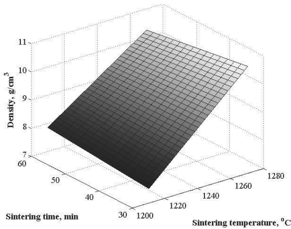
Fig. 12. RFP describing relationship between density and the temperature, and sintering time, for GM-90HSS/10WC, sintered in furnace with the atmosphere of the N_2+5\% H_2
