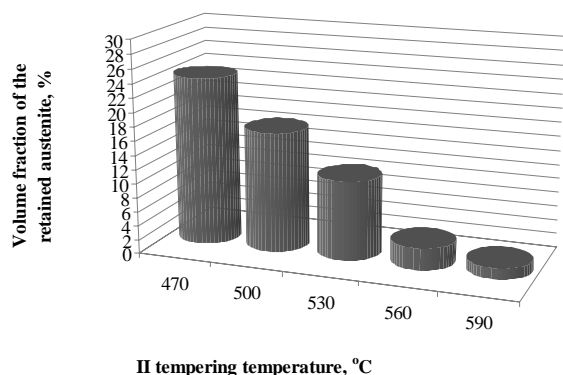
Fig. 47. Relationship between the volume portion of the retained austenite with the second tempering temperature in the GM-100HSS substrate layer of GM-75HSS/25WC hardened at the temperature of 1210°C after austenitising for 120 s
