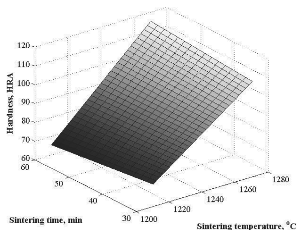
Fig. 19. RFP describing relationship between hardness and the temperature, and sintering time, for GM-75HSS/25WC, sintered in the furnace with the atmosphere of the flowing N_2+5\% H_2
