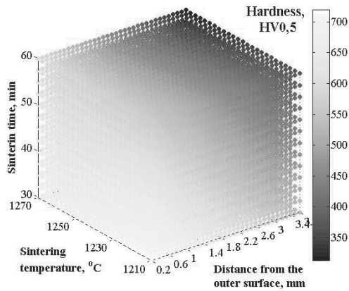
Fig. 22. RFP describing relationship between hardness HV and the distance from the outer surface, temperature, and sintering time, for GM-90HSS/10WC, sintered in the furnace with the atmosphere of the flowing N_2+5\% H_2
