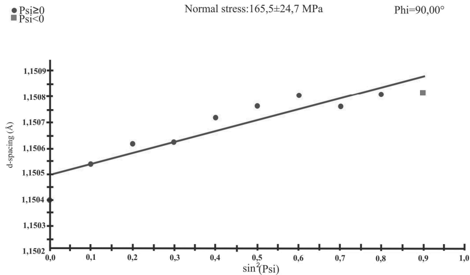
Fig. 56. Changes in the interplanar distance value of d reflex (201) according to \sin^2\psi sintering temperature of 1460°C; results for the GM-3Co/97WC surface layer
