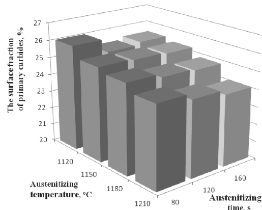
Fig. 44. Relationship between the surface portion of carbides in the GM-100HSS substrate layer of hardened GM-75HSS/25WC and austenitising conditions
