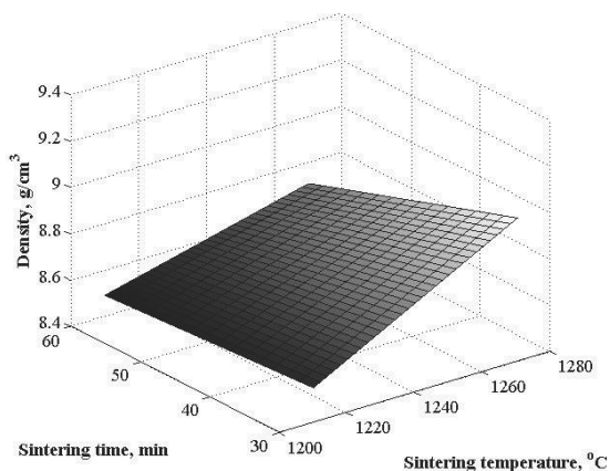
Fig. 10. RFP describing relationship between density and the temperature, and sintering time, for GM-75HSS/25WC, sintered in the vacuum furnace
