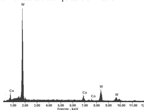
Fig. 49. Diagram of intensity according to energy of scattered X-ray radiation for the whole area for the surface layer
