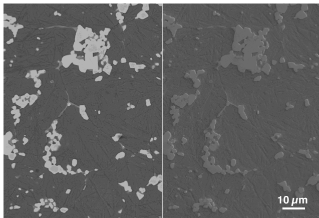
Fig. 41. Structure of the quenched and twice tempered GM-95HSS/5WC intermediate layer
