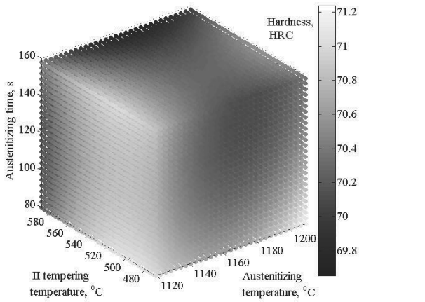
Fig. 36. RFP describing relationship between hardness and the temperature, and austenitising time, and second tempering temperature for the GM-75HSS/25WC surface layer
